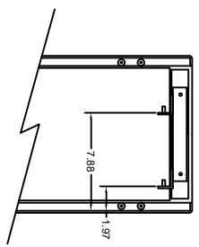
ADJUSTABLE MOUNTING PLATE
