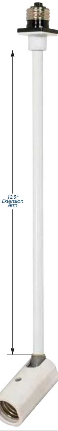
77-621 Recessed light converter 13.25" overall height Packing: 6/Master, 1/Card
