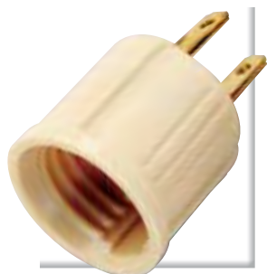
90-438 Ivory Medium Base – Polarized Socket Outlet Adapter 660W-125V
