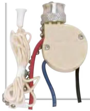
S70-689 Pull chain fan switch, 2 circuit low, med., high & off 1/8 IP threaded Packing: 72/Master, 6/Inner
