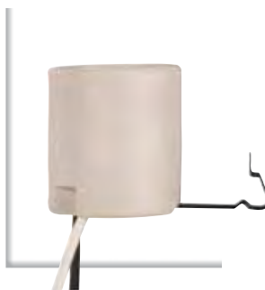
80-1220 Snap-In Socket Bracket Extends 1" from End of Socket 12" AWM B/W Leads 150°C 660W-250V
