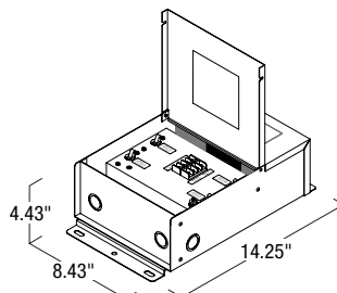
NMT-244/12C2D1: 120/12V 240W C2 Dimm. Driver
