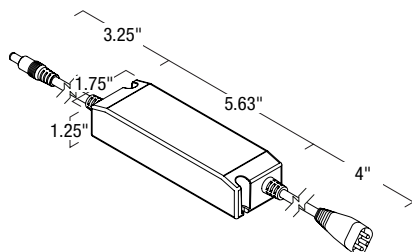
NAPK-530HW/12: 12V 30W Class II Hardwire Driver
