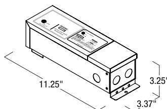
NMT-36/12C2D1: 120V/12V 36W C2 Dimm. Driver
