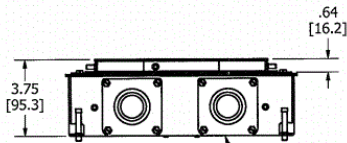
END VIEW KO PLATES
