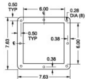
6 x 6 Top and Bottom Flange D35
