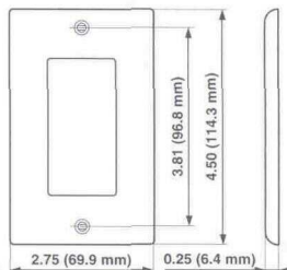
NYLON WALLPLATE Cat. No. 80401-N
