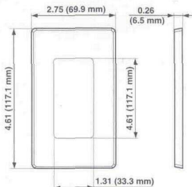
SCREWLESS SNAP-ON WALLPLATE Cat. No. 80301
