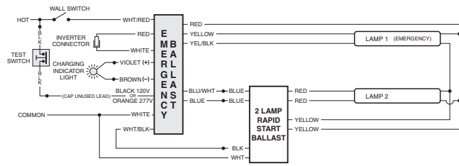
FIG D TWO (2) LAMP RAPID START BALLAST
